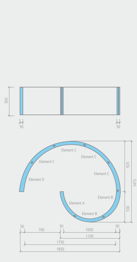
Fundo Nautilo, extension collar
