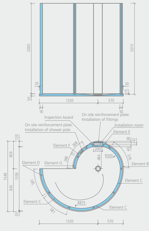
Fundo Nautilo libero , designer shower
